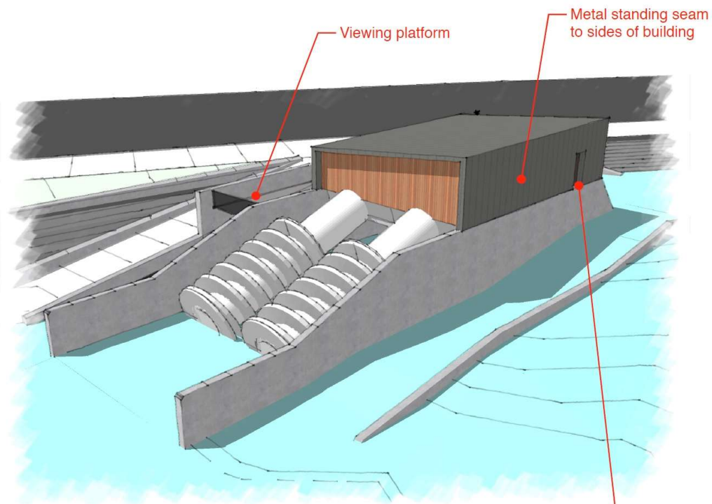
Tiverton Micro Hydro Power Building Option 2. Standing Seam Wrap Over. Fox Ecological Architects. April 2020.
