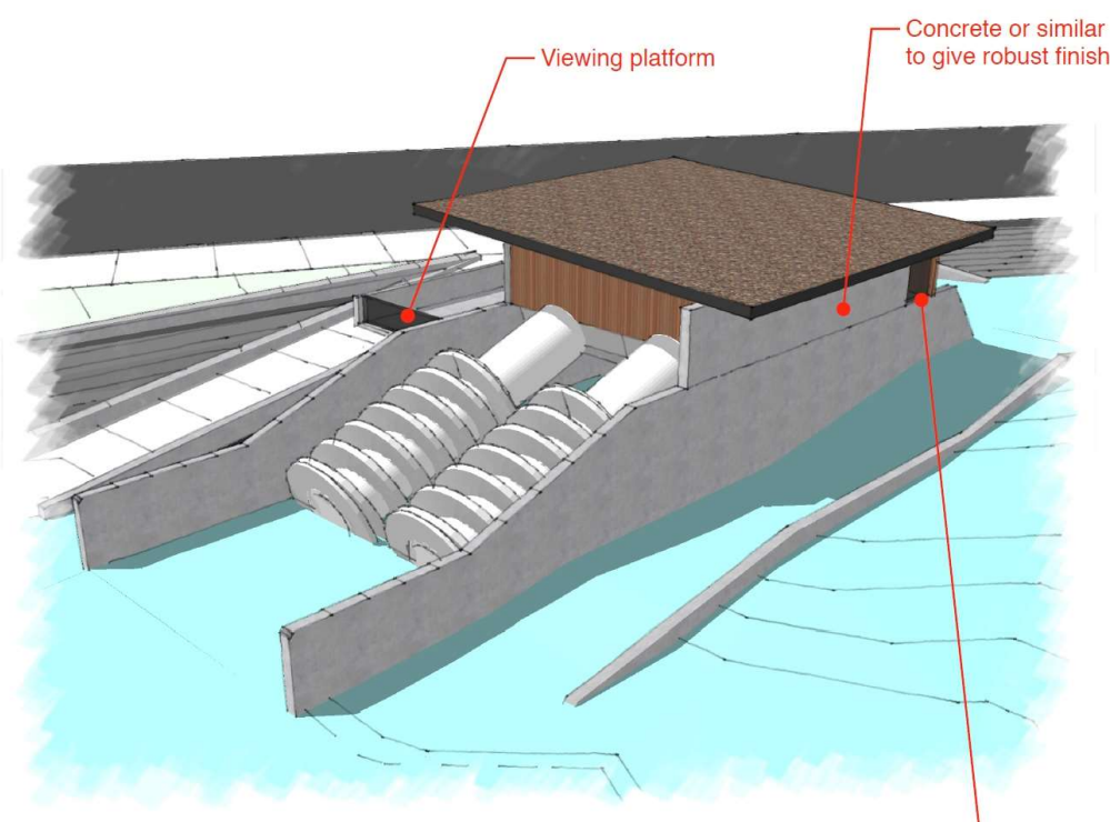
Tiverton Micro Hydro Power Building Option 3. Green / Gravel Roof. Fox Ecological Architects. April 2020.
