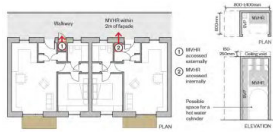
MVHR systems are an effective way of providing ventilation to airtight homes. The unit should be located within 2m of the façade (Source: Levitt Bernstein + Etude)
